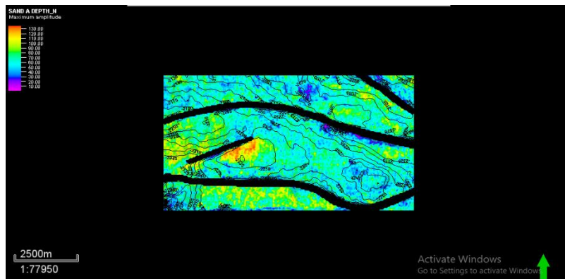
Figure 14: Maximum Amplitude Attribute for Sand A
