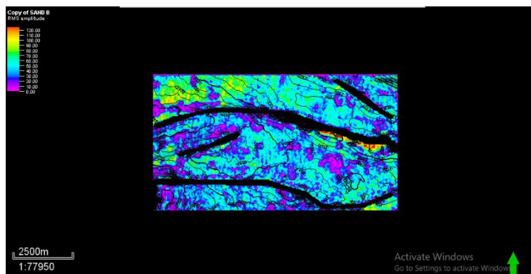
Figure 11: RMS Amplitude Attribute for Sand B
