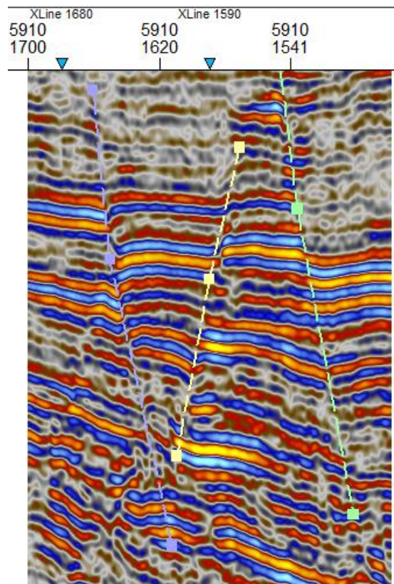
Figure 6: Picked Fault Stick on Seismic Inline
