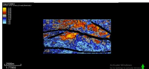
Figure 25: Sweetness Attribute for Sand D
