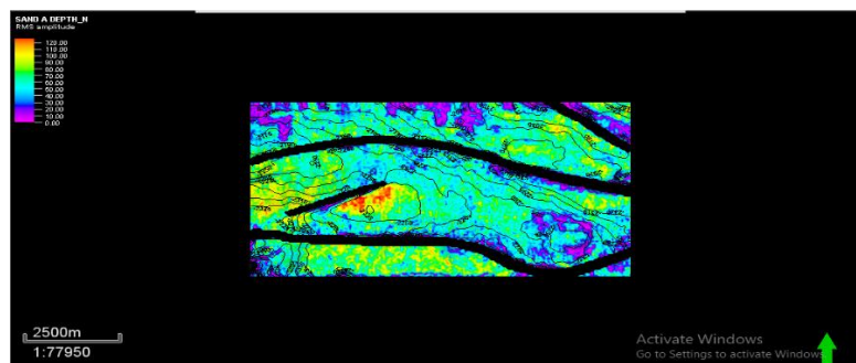
Figure 10: RMS Amplitude Attribute for Sand A
