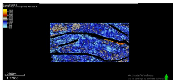
Figure 23: Sweetness Attribute for Sand B
