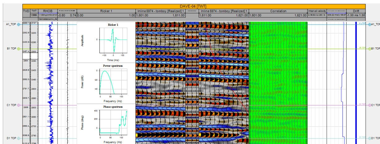
Figure 8: Synthetic Seismogram
