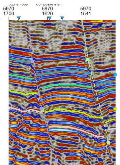
Figure 9: Four Horizons Identified for Each Sand Zone Across the Seismic
