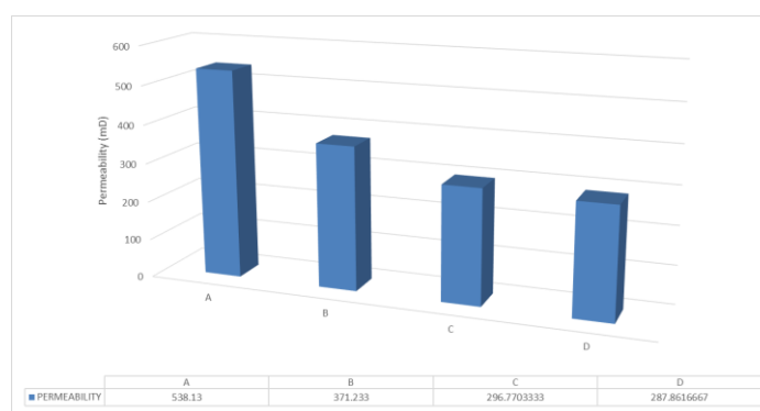
Figure 4: Graphical Plot of Average Permeability in Sand A, B, C, and D
