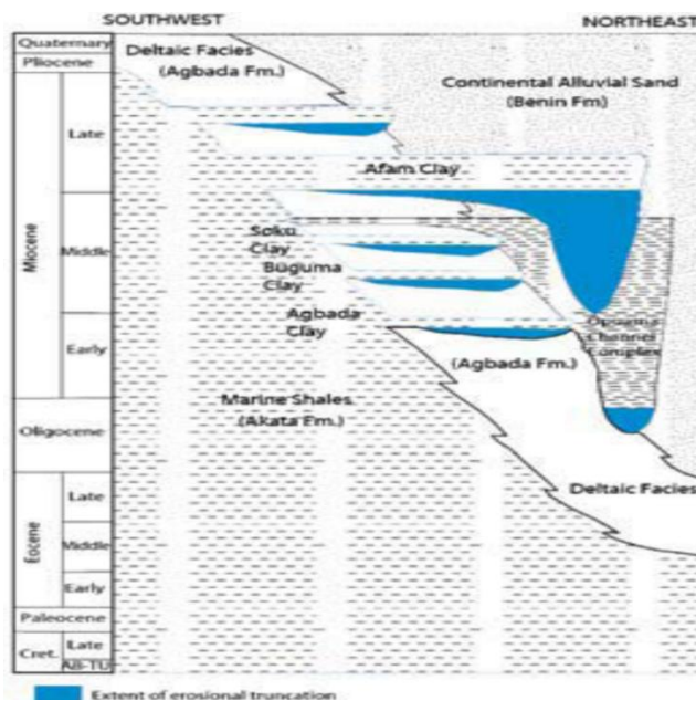
Figure 1b: Stratigraphic Column Showing the Three Formation of Niger Delta (Short and Stauble, 1967)
