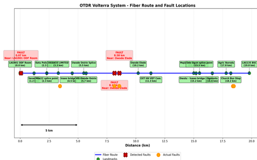
Figure 1: Fibre Route and Fault Location Map for the Proposed OTDR Volterra System, showing 17 Geographical Landmarks, Detected Faults (red x), and Verified Fault Positions (Solid Orange Circles) Along a 20-km Route in Lagos, Nigeria
