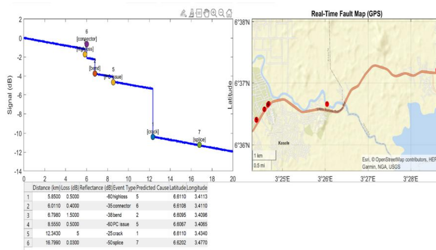
Figure 3: Real-time OTDR Monitoring and Geographical Fault Localisation Using the Proposed VAF System
