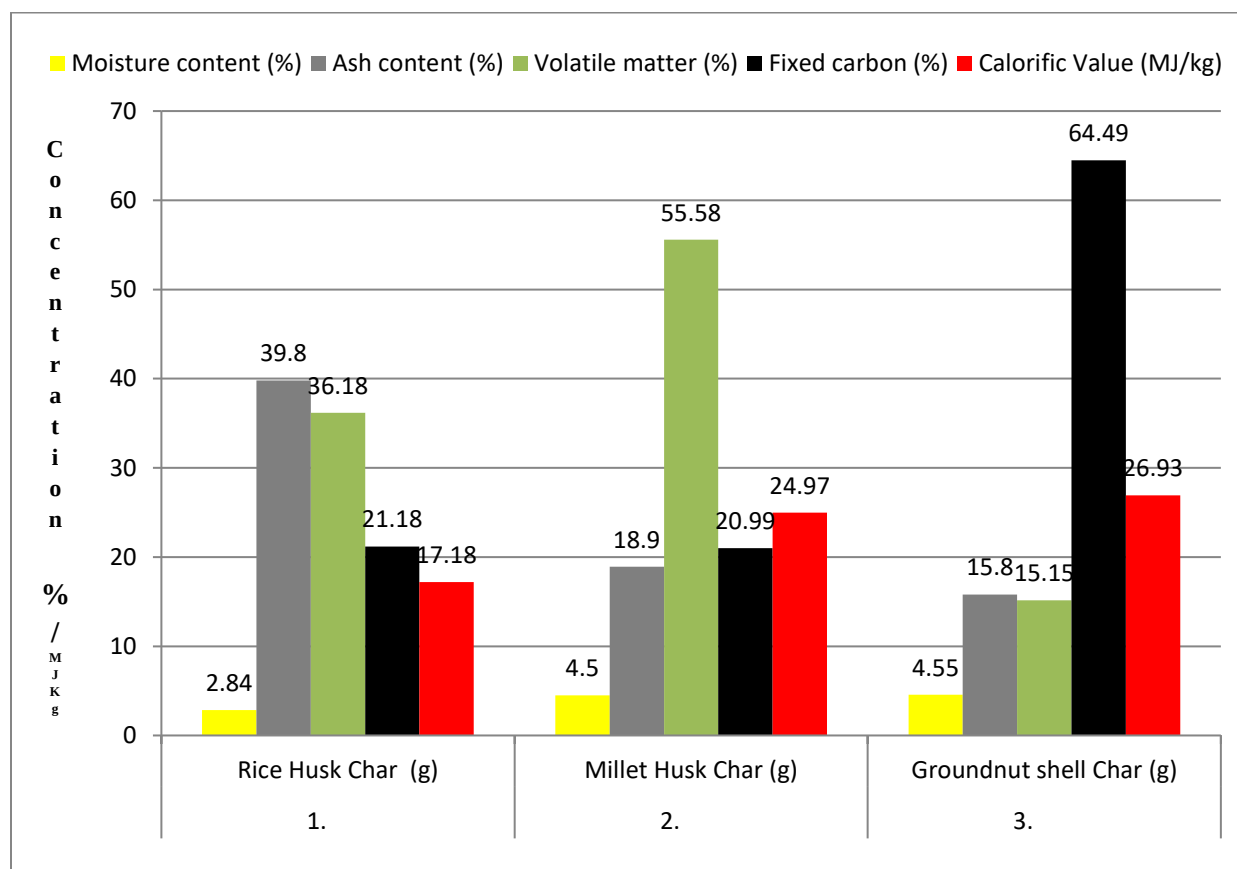
Figure 2: Chart showing Variations in Physical Parameters of Biochar
