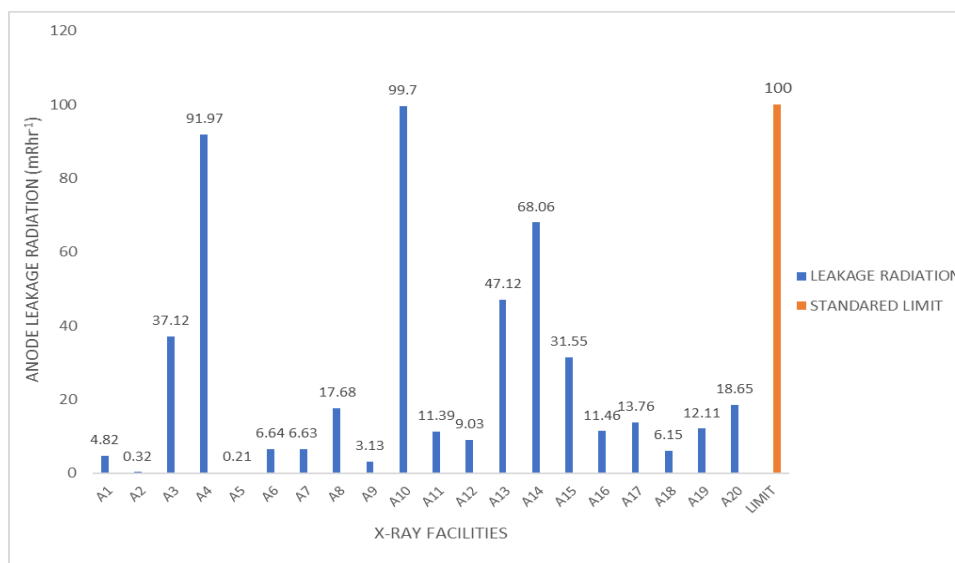
Figure 2: Comparison of the Anode Side Leakage Radiation to Standard Limit
