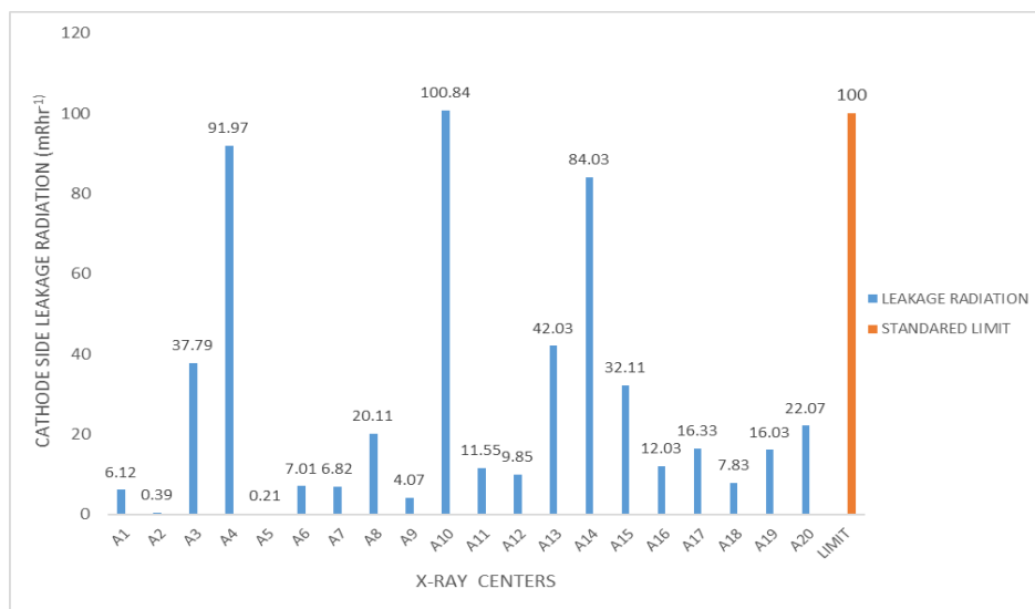
Figure 1: Comparison of the Cathode Side Leakage Radiation to Standard Limit
