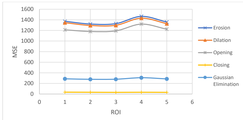
Figure 4: Performance of filter based on MSE
